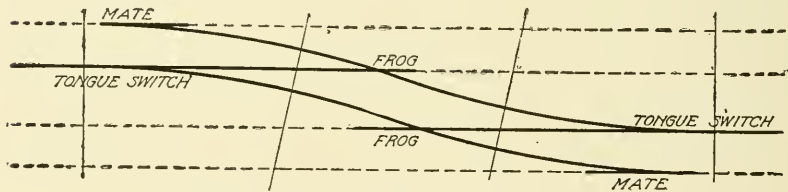
Fig. 234. Standard Right-Hand Cross-Over
